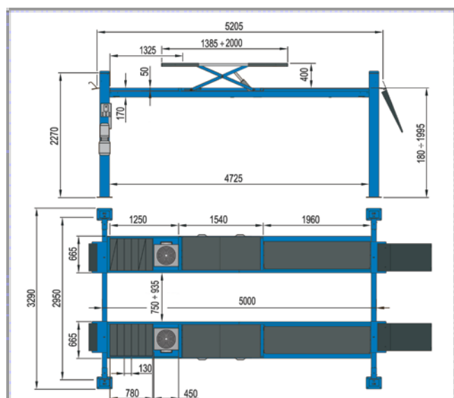
P4C 450 CT LT EVO
